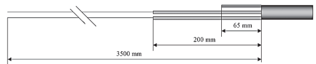
4.2.17 Remove the outer cable jacket over a distance of 3500 mm starting from the side term plate and cut the strength member at 65 mm from the cable jacket.
