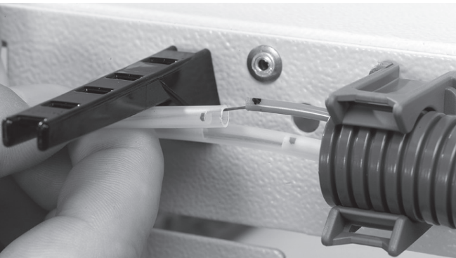
4.1.13 Select a loose tube and slide a 75mm long FOPT-CT over the transportation tube and loose tube or the transportation tube directly over the loose tube.
