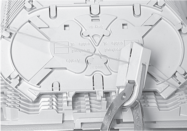
5.19 Make sure the transition of secondary to primary coating is in the splice protector. If this is not possible: strip the secondary coating (semi-tight) in the middle of the groove plate.
