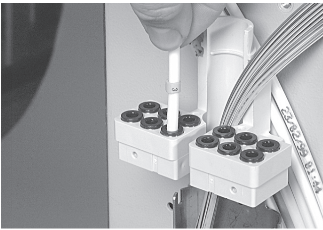
4.1.29 Insert the tubes in the connectors. Use 6 positions at the left when cable is mounted at the left side of the bracket.
