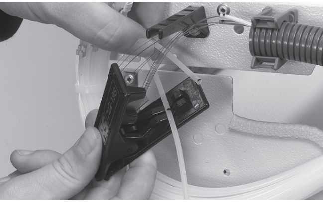
4.1.12 Strip the loose tubes from the mark and cut the overlength of the transportation tubes. Clean the fibers very well to make feeding easier.
