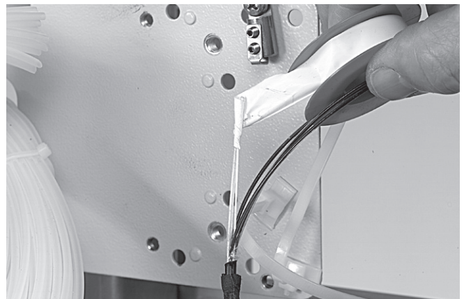
4.2.20 Wrap some layers of teflon tape around the ends of the strength members to keep them together.
