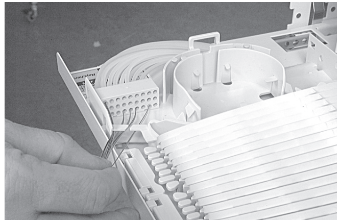
4.1.15 Pull the fibers at the other end of the tubes.
