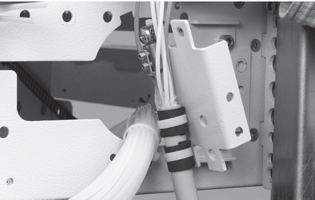
4.2.3 Strip the cable over 3,5 m. Cut the strength member at 35 mm from the outer jacket. Apply foam tape at the tie wrap positions. Install the prepared cable on the side termination plate.
