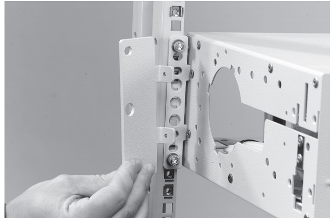
3.1.5 If necessary mount the adaptation brackets 19"-ETSI (FIST-MB2-M or FIST-MB2-M-AS).
