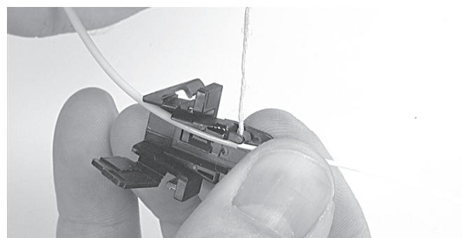
5.10 In case of less kevlar (typically this means pigtail diameter < 2,3 mm); wrap the kevlar to ensure a good strain relief.
