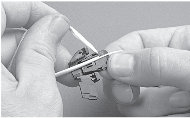
5.7 In case of 2 pigtails/KTU; identify 1 of the fibers with a marking pen.
