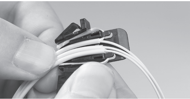
5.11 Installation of first and second pigtail at the same side of the KTU.
