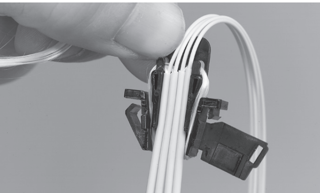
5.12 Installation of third and fourth pigtail at the opposite side of the KTU.
